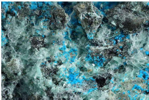
\text{Ca}(\text{V}^{4+}\text{O})_2(\text{AsO}_4)_2(\text{H}_2\text{O})
